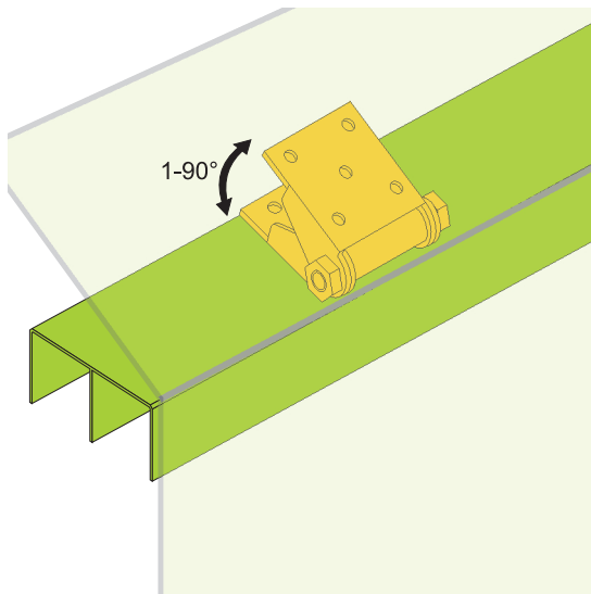
uchwyt do mocowania toru górnego pod skosem fastening to upper rail installed to sloping ceilings
